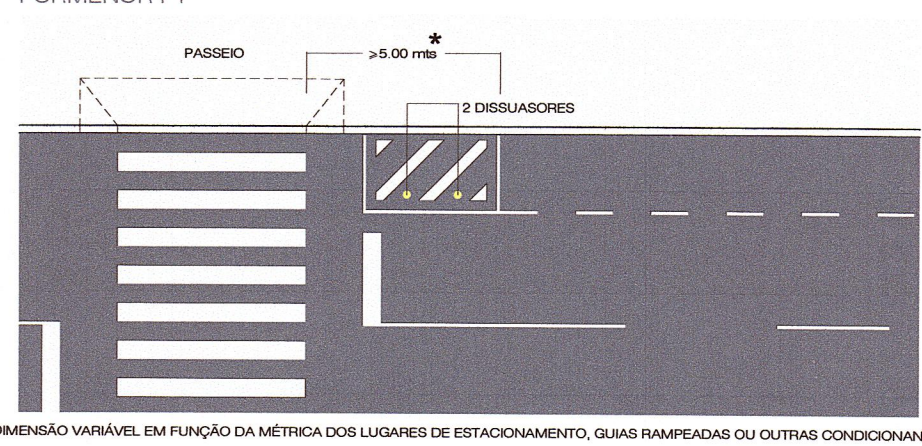
PORMENOR P1
