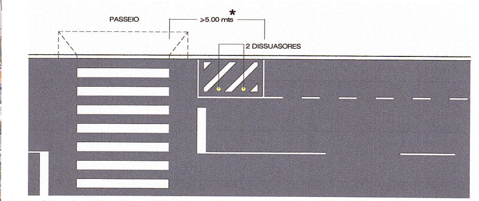
PORMENOR P1
